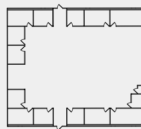
82'x75' Communications Building
