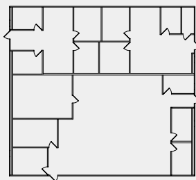
75'x68' Plans & Operations Building
